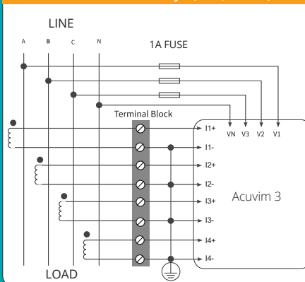
3 Element 4 Wire Wye (3LN, 3CT**)
