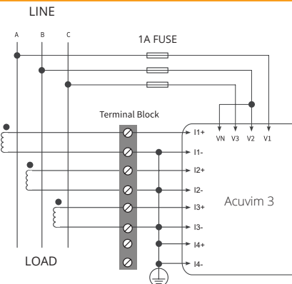
2 Element 3 Wire Delta (2LL, 3CT)
