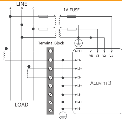
2 Element 3 Wire Delta with PT (2LL, 2CT)
