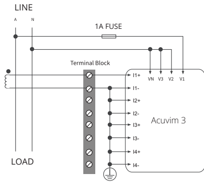
1 Element 2 Wire (1LN, 1CT)
