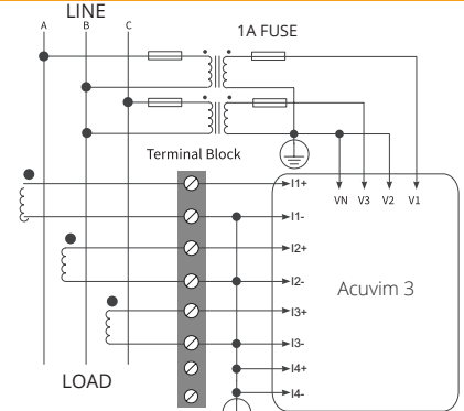
2 Element 3 Wire Delta with PT (2LL, 3CT)
