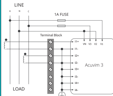
2 Element 3 Wire 1 Phase (1LL, 2CT)
