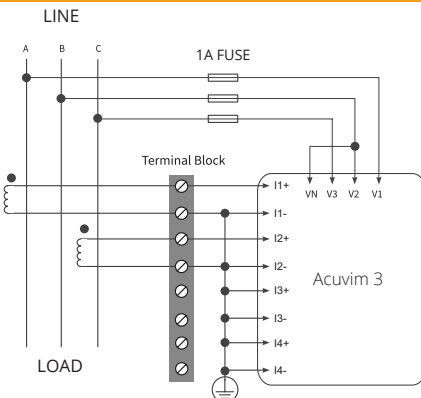
2 Element 3 Wire Delta (2LL, 2CT)
