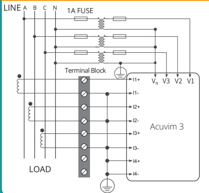
3 Element 4 Wire Wye with PT (3LN, 3CT)
